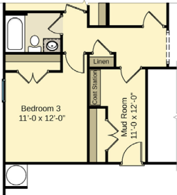
Mud Room 1/4" = 1'-0" (NO STAIRS / BONUS ROOM)
